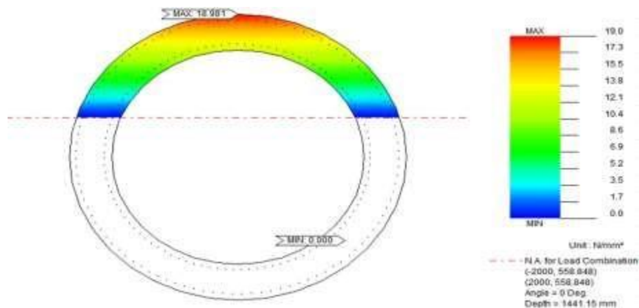
Figure 9: concrete stress values under SLS rare load combination (output from MIDAS GSD)
